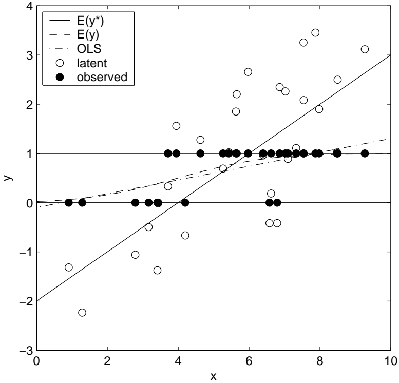
Figure 2: The probit model with a latent variable. N = 30 , K = 2 , \beta_0 = -2 and \beta_1 = 0.5 .
